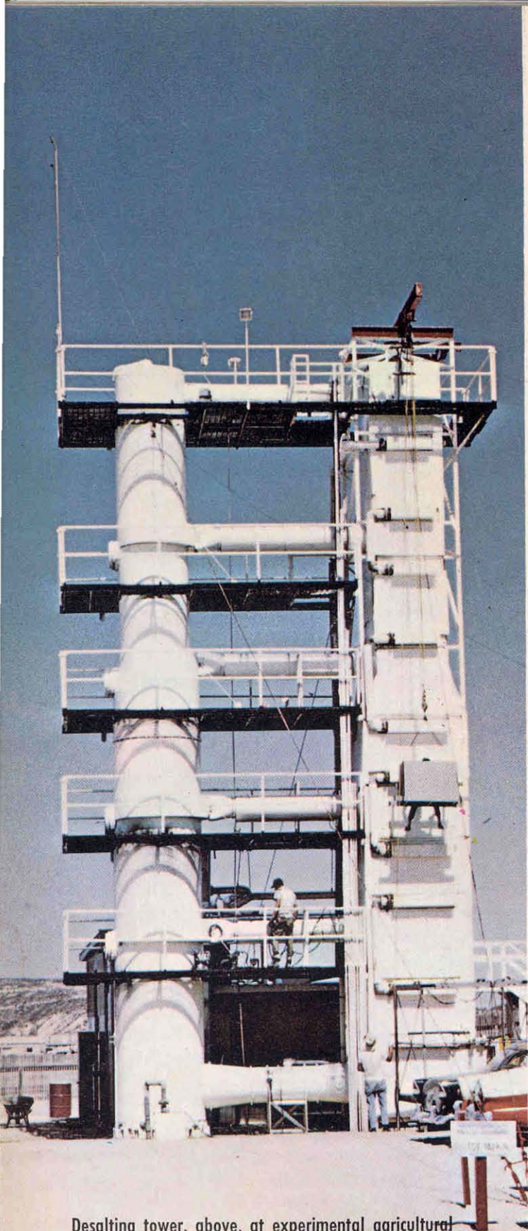
Desalting tower, above, at experimental agricultural project at Puerto Peñasco, Sonora, Mexico, on arid Gulf of California coast. Desalted seawater is used for growing variety of plants in greenhouses of inflated plastic, opposite page.
