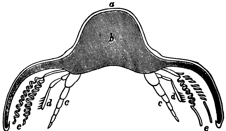
Complex transverse section of a Trilobite (after Wolcott). a, dorsal crust; b, visceral cavity; c, legs; d, epipodite (structure to keep gills clean and maintain fresh water circulation); e, spiral gills.
